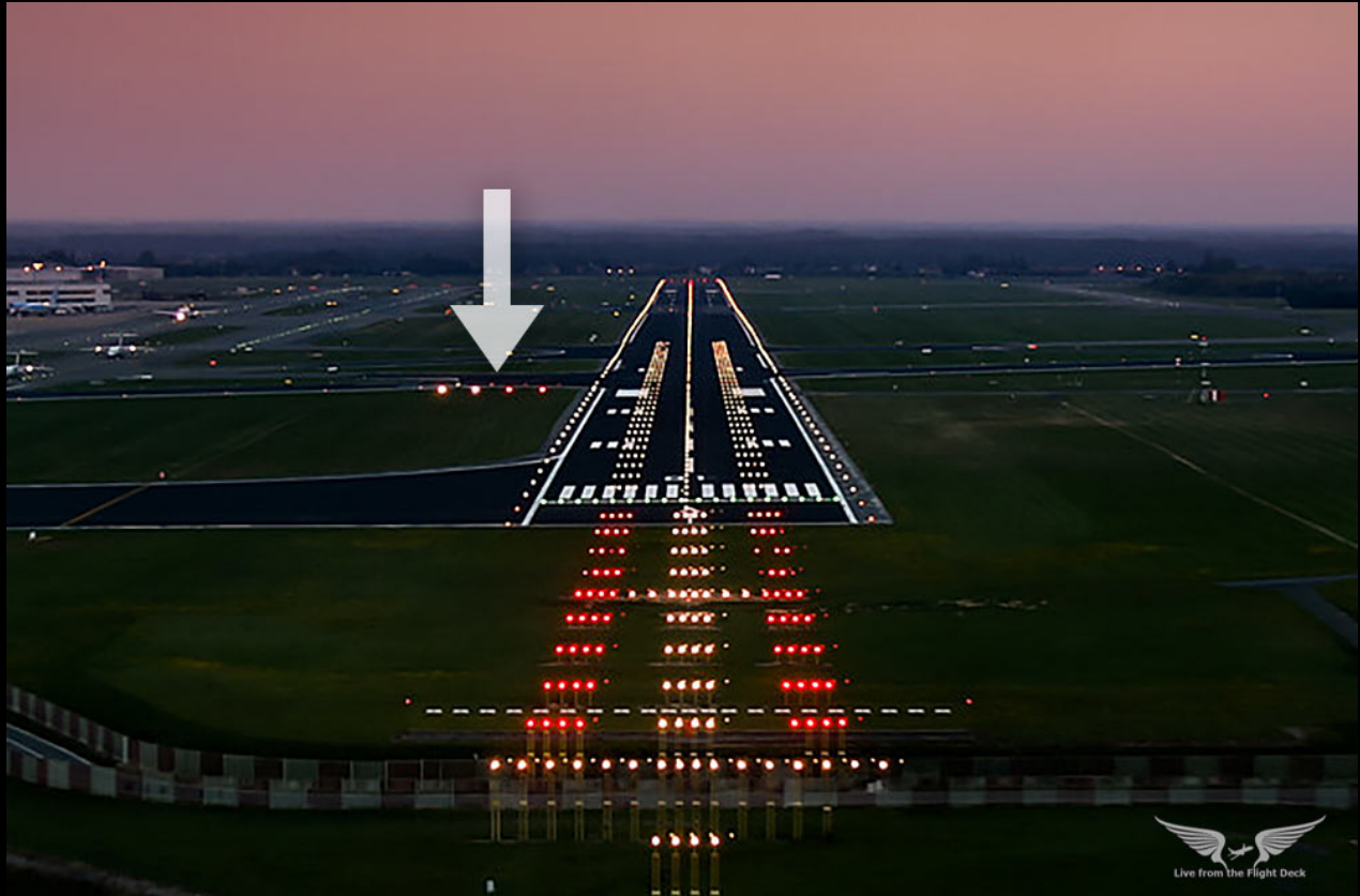
Figure 60 – Traditional PAPIs
